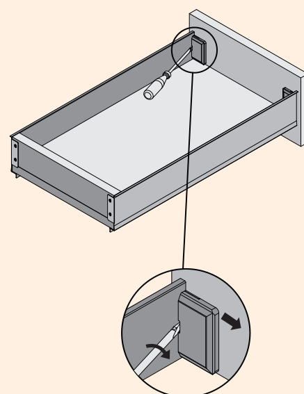
Cover Cap Assembly & Removal
