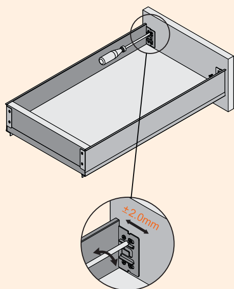
Adjustment Direction & Tolerance
